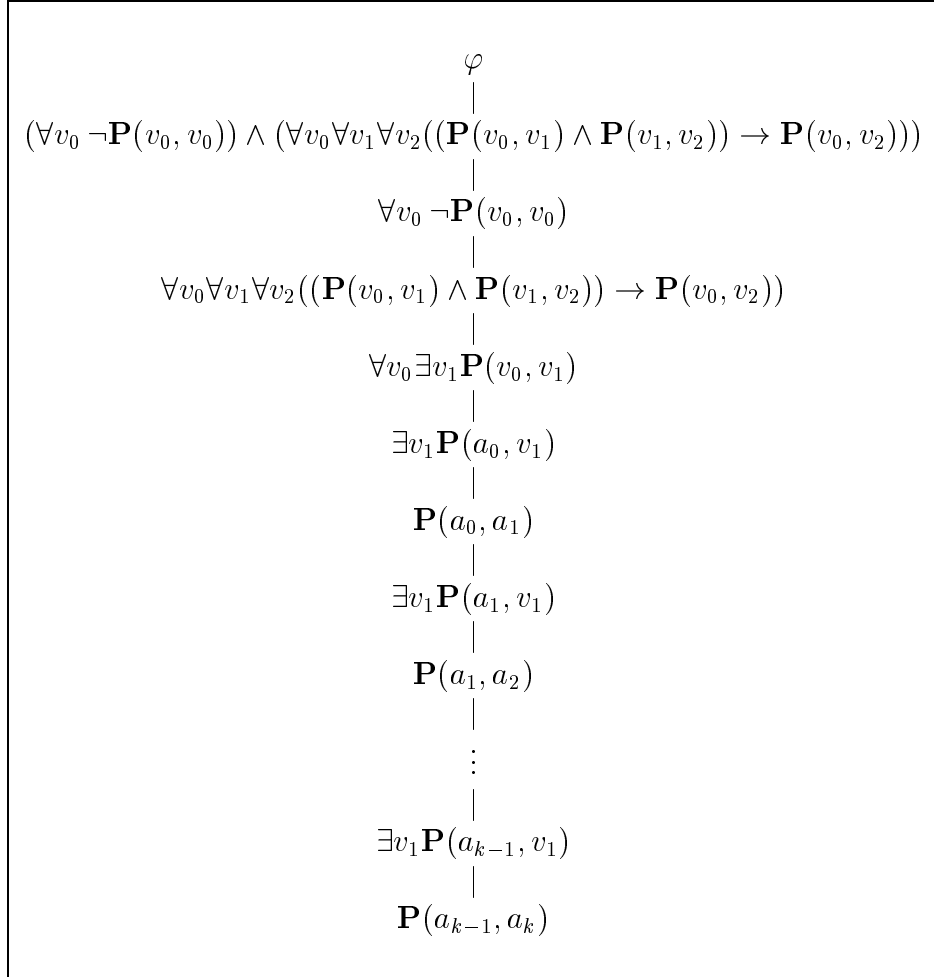
Figura 2.2: \mathcal{A}_{4+2k}
