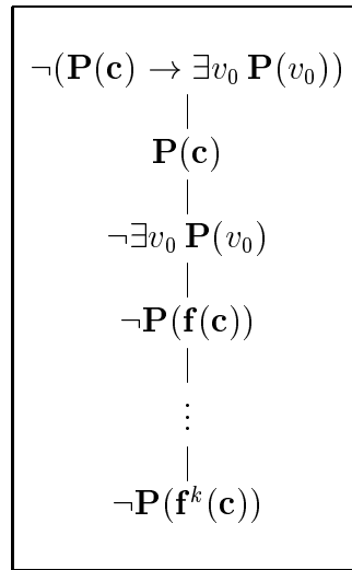
Figura 2.4: \mathcal{B}_{2+k}
