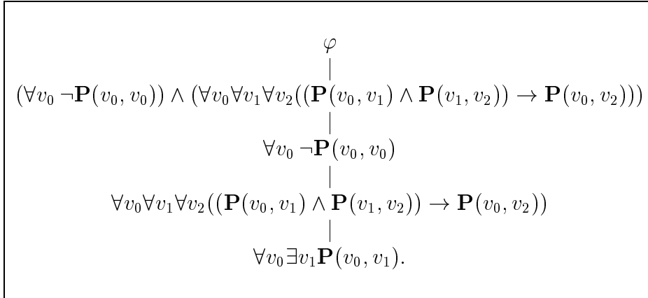
Figura 2.1: \mathcal{A}_4
